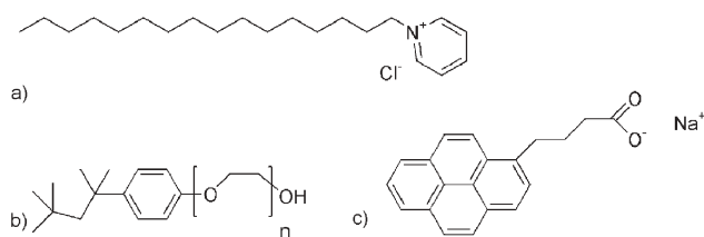
Scheme 5 Structures of surfactants used for PL studies of nanotube dispersions in water (a) CPCI, (b) Triton X-100 and (c) SPB.
